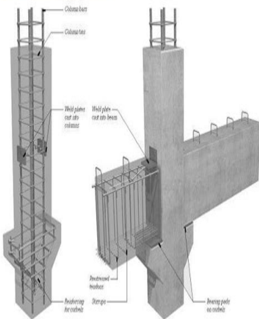
BEAM TO COLUMN CONNECTION
