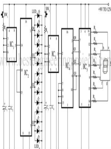
Figure 2 Circuit Diagram of Electronic Number Scoring Game
